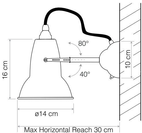
Original 1227 Wall Light shown
